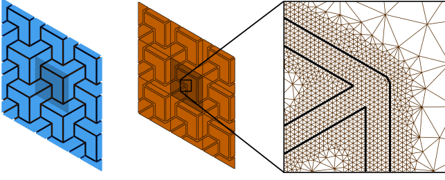
Fig. 2. Scale ( left ) and substrate ( middle ) meshes are generated from isohedral tilings. To facilitate coupling, the substrate is meshed such as to conform to the boundaries of the scale mesh ( right ).
