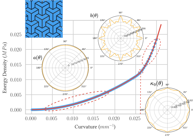
Fig. 4. Macro-scale parameters a(\theta) , b(\theta) and contact curvature \kappa_0(\theta) for a fitted circular harmonics (Eq. 11) are shown in orange. The blue dots in the energy density-curvature plot are sample points from the native scale simulation and the red line is the fitted piecewise-quadratic unidirectional energy density (Integral of Eq. 10) with slopes a and b and regime switch point k_0 .
