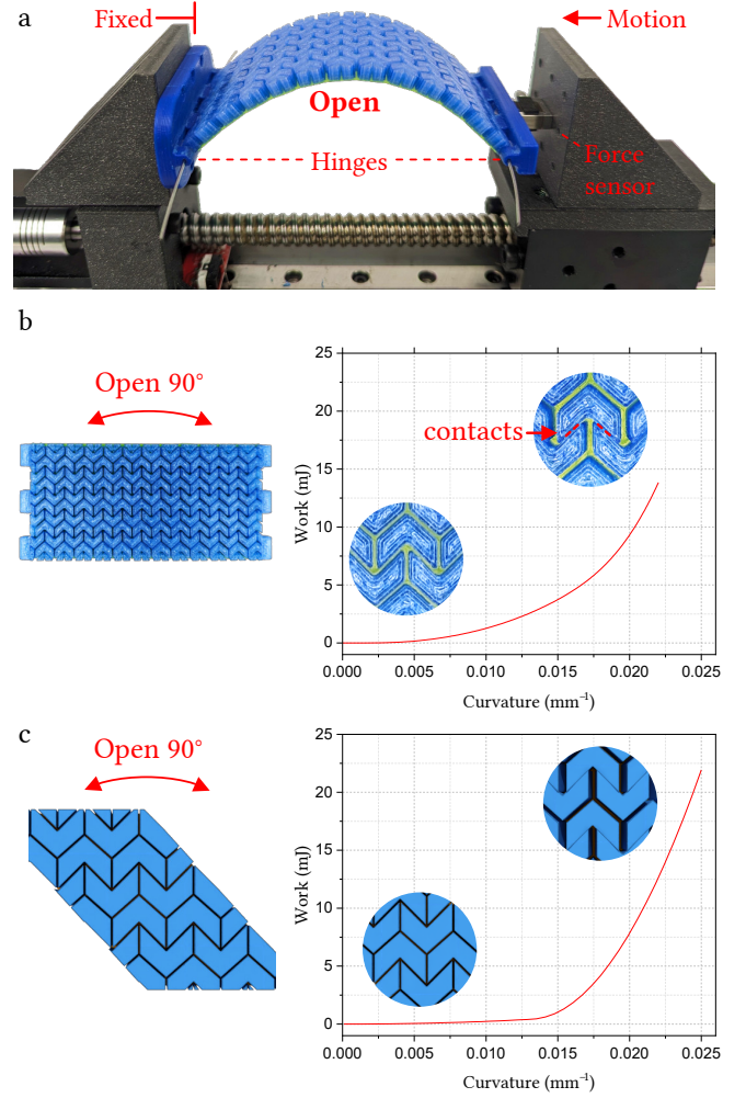
Fig. 11. Contact-induced stiffening for opening curvatures, using the same setup as in Fig. 10. (b) We record force-displacement behavior for opening curvatures of an arrow-like pattern, revealing contact induced stiffening ( red curve ) due to non-convex interlocking scales. (c) Our native-scale simulation reproduces the contact patterns and shows good qualitative agreement with experimental results.
