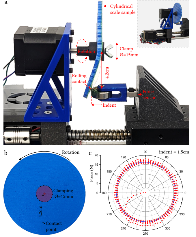
Fig. 6. Experimental setup for omnidirectional measurement of force-displacement response. Top: A disc-shaped sample is mounted onto a mandrel rotating at constant speed. A force probe imposes constant displacement at the boundary of the sample. Bottom: A 3D-printed solid disc is used for calibration. Force is recorded for 6 consecutive revolutions.
