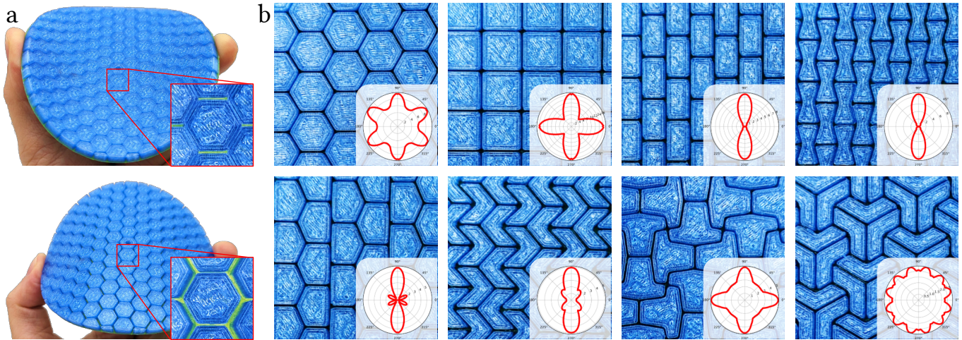
Fig. 1. Flexible scaled sheets offer a unique and intriguing combination of strength and flexibility. a : Bending-induced contact between scales leads to distinct behavior for positive ( top ) and negative ( bottom ) curvatures. b : our homogenization approach enables us to capture the macro-mechanical curvature response of arbitrary scale patterns.
