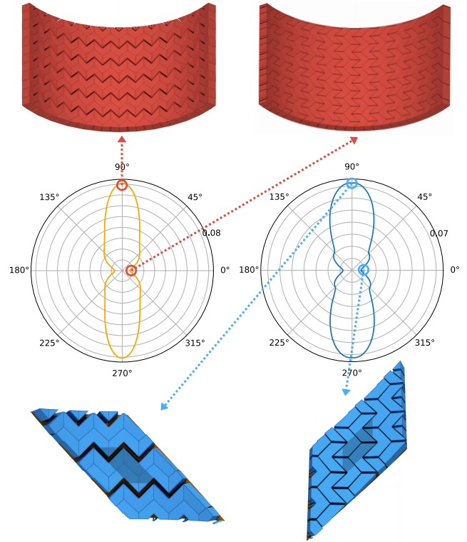
Fig. 14. Directional bending energy density for simulations using our macro-mechanical model for a 100\text{mm} \times 50\text{mm} rectangular sheet (red) compared against native-scale simulations with enforced periodic boundary conditions (blue). All simulations are run at a curvature of 0.02\text{mm}^{-1} .
