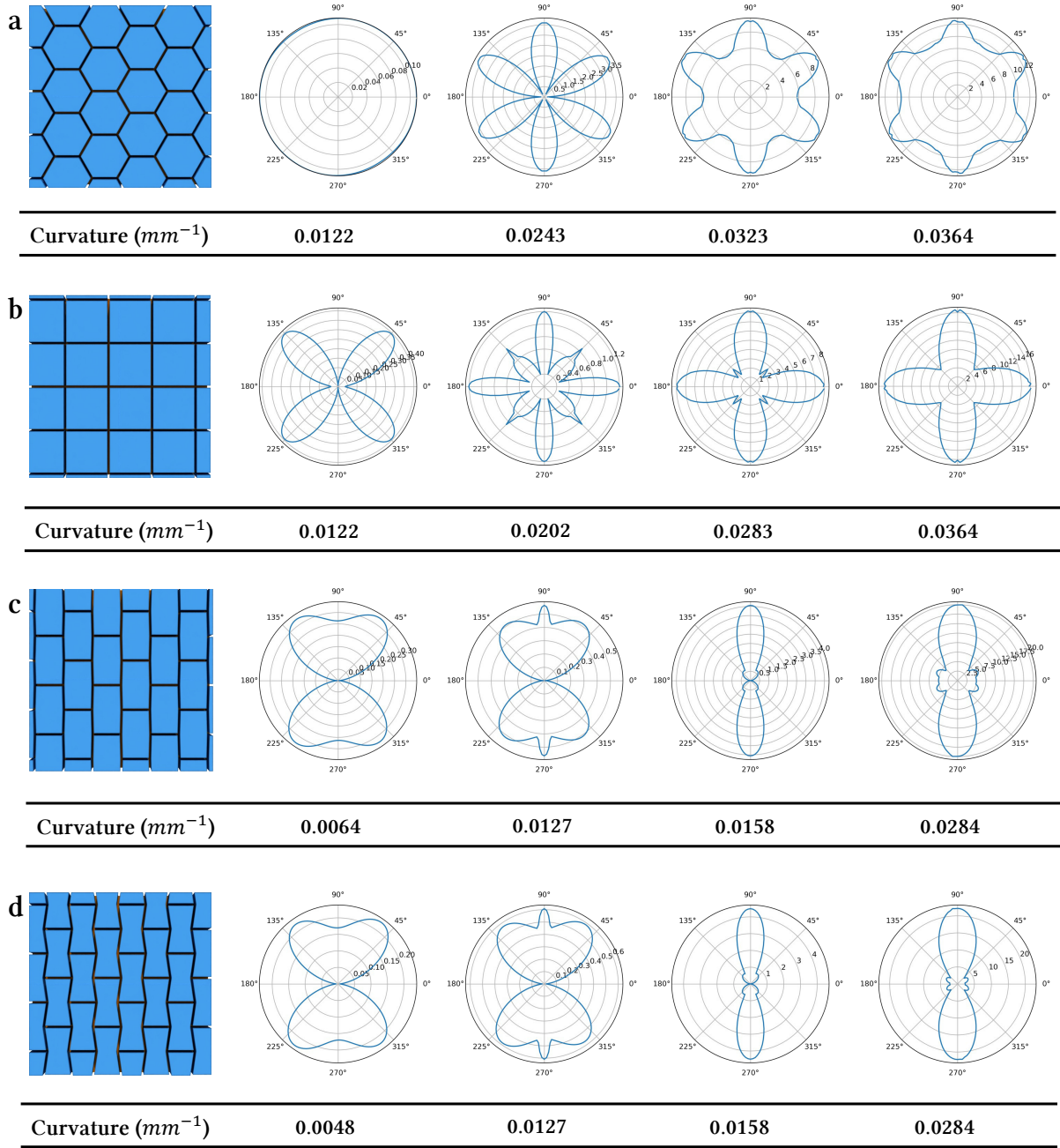
Fig. 7. Native-scale simulations, part 1. We show moment-curvature plots (columns 2-5) for increasing curvature values on a set of patterns (column 1).
