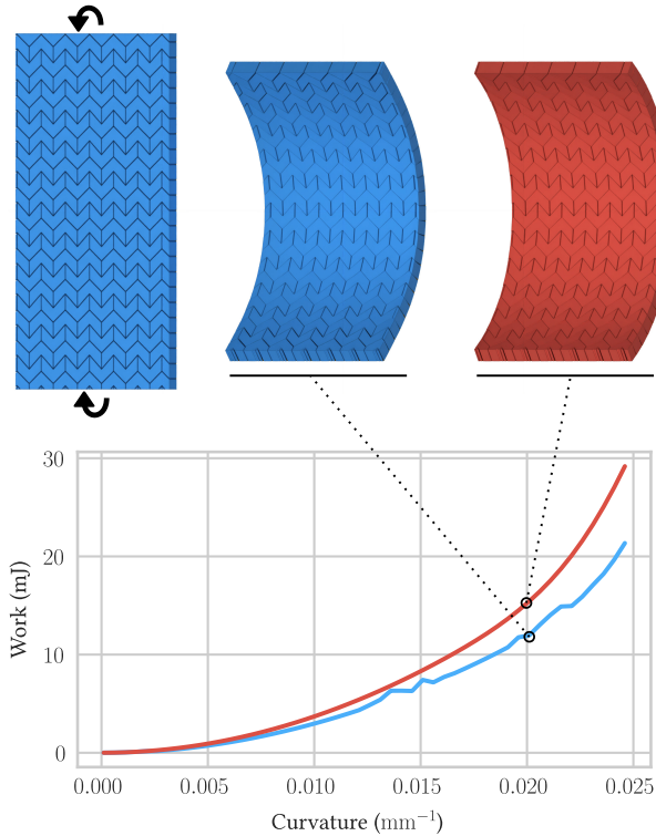
Fig. 13. Bending simulation of a 100\text{mm} \times 50\text{mm} rectangular sheet covered with arrow-shaped scales using the native-scale model (blue) compared against a shell simulation using the fitted macro-mechanical model (red).
