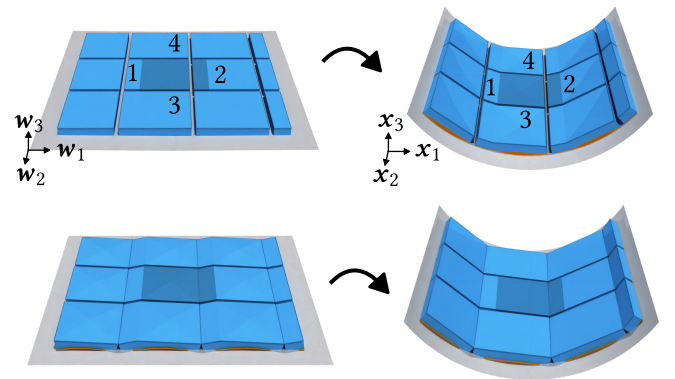
Fig. 3. Mapping from curvilinear space ( left ) to world-space ( right ) as described through Eq. (2). Top : a planar initial state leads to curved scales and high elastic energy in world-space. Bottom : curvilinear coordinates are optimized such as to minimize energy when mapped to world-space.
