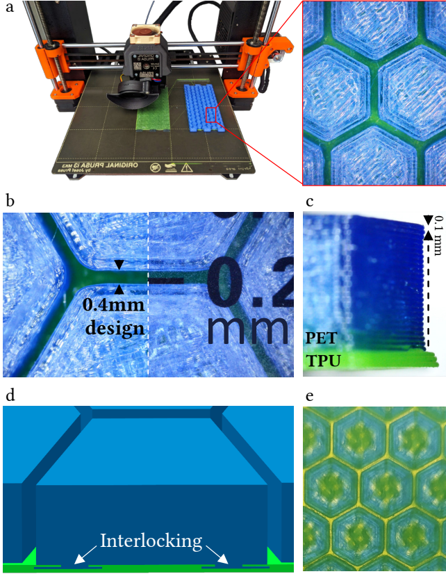
Fig. 5. We manufacture prototypes using 3D printing (a). The gap between scales (0.4mm) was controlled and straight edges with slightly rounded corners were observed (b). Layers of 0.1mm were used to print both the TPU substrate and the PET scales on top (c). An interlocking pattern was added to enhance adhesion between substrate and scales (d). Scales were filled using a gyroid pattern (e).
