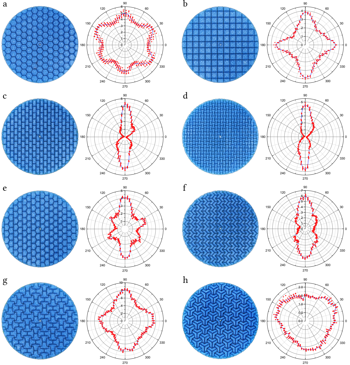
Fig. 9. Experimental characterization of scaled sheet materials using our omnidirectional bending setup (Fig. 6). We impose 1.5cm indentation at the boundary of each disc-shaped sample and plot the resulting force at equally-spaced sample locations for 6 full revolutions. Measured data is indicated in red, blue curves show averages of the 6 samples per direction.
