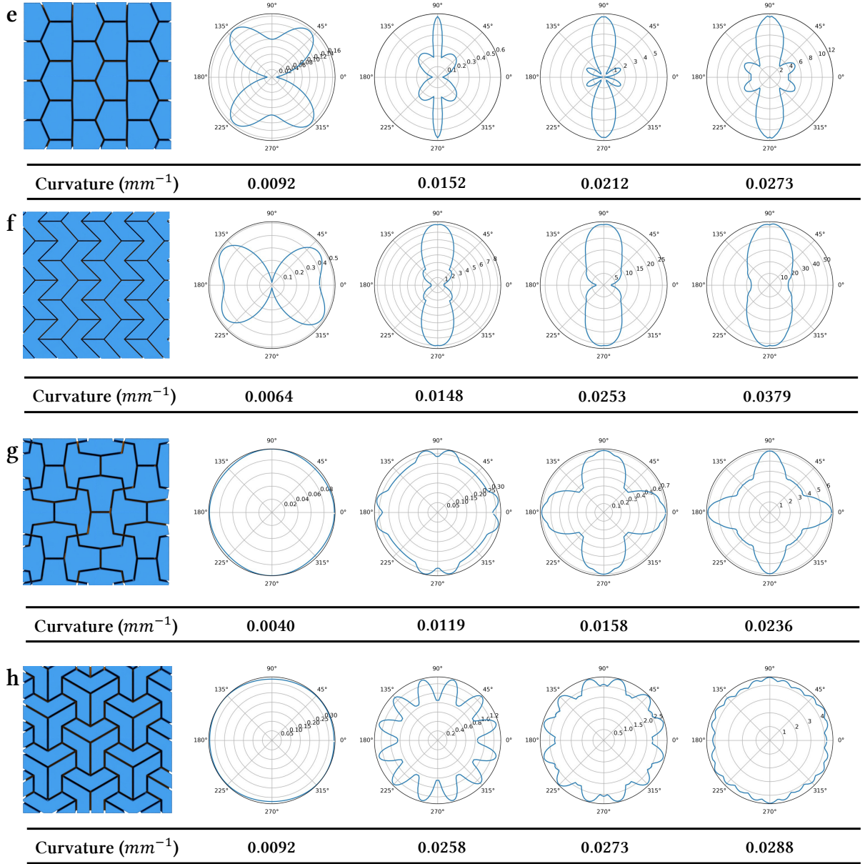
Fig. 8. Native-scale simulations, part 2. We show moment-curvature plots (columns 2-5) for increasing curvature values on a set of patterns (column 1).
